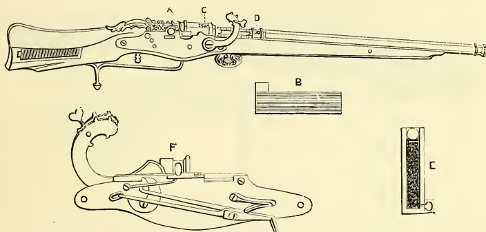
Breech-loading Arquebus of King Henry VIII.
